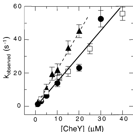
FIGURE 4: Analysis of the effect of CheY concentration on the kinetics of phosphotransfer from P-CheAΔP2 to CheY and from P-CheA 1-139 to CheY. For the reaction between CheY and P-CheAΔP2, the plotted k_{\text{obsd}} values are the pseudo-first-order rate constants derived from rapid quench (□) and stopped-flow (●) experiments (as in Figures 2 and 3). The best-fit linear relationship defined in this plot (solid line) indicates a second-order rate constant of 1.5 \times 10^6 \text{ M}^{-1} \text{ s}^{-1} for the reaction between CheY and P-CheAΔP2. For the reaction between CheY and P-CheA 1-139 , the plotted k_{\text{obsd}} values (▲) were determined by stopped-flow experiments. The best linear fit (dashed line) of these data indicates a second-order rate constant of 2.3 \times 10^6 \text{ M}^{-1} \text{ s}^{-1} . Error bars indicate standard errors of the mean.
