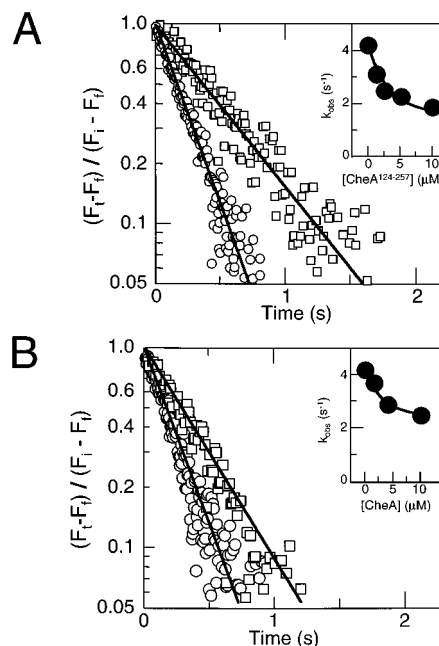
FIGURE 5: Effect of CheA 124-257 and wild-type CheA on the rate of phosphotransfer from CheAΔP2 to CheY. Panel A: reaction mixtures contained 0.25 μM P-CheAΔP2, 2.8 μM CheY, and either no CheA 124-257 (○) or 10 μM CheA 124-257 (□). The inset shows the relationship between the observed first-order rate constant ( k_{\text{obsd}} ) and the concentration of CheA 124-257 . Panel B: reaction mixtures contained 0.25 μM P-CheAΔP2, 2.8 μM CheY, and either no wild-type CheA (○) or 10 μM wild-type CheA (□). The inset shows the relationship between the observed first-order rate constant ( k_{\text{obsd}} ) and the concentration of CheA. In both panels, reaction time courses were monitored using fluorescence emission changes as in Figure 3. The data are presented as normalized semilog plots because the reactions in the presence of CheA 124-257 or wild-type CheA exhibited smaller amplitudes than did reactions in the absence of these additions [as expected because of the quenching of CheY intrinsic fluorescence associated with CheY binding to the P2 module of CheA (38)]. F_i , F_t , and F_f denote the fluorescence emission intensity observed at t = 0 , t = \text{time } t , and at the end point of the reaction, respectively. The solid lines in the main panels represent the computer-generated best fits of each time course to a single exponential. The solid lines in the insets depict the inhibition pattern expected if the CheY·P2 complex has a K_d of 1.5 μM and a phosphotransfer activity that is 30% that of free CheY.
