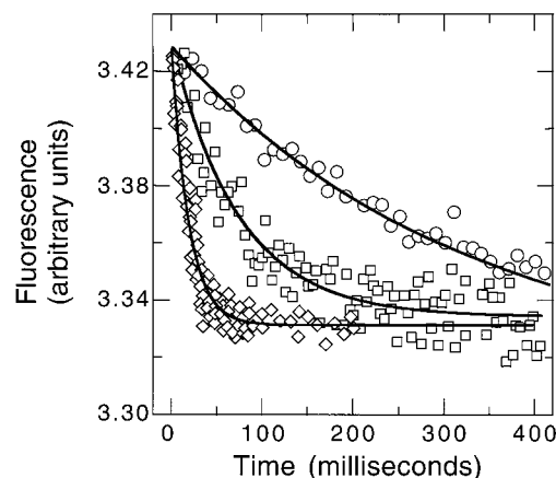
FIGURE 3: Time course of fluorescence changes following mixing of P-CheAΔP2 with CheY. P-CheAΔP2 (0.25 μM) was mixed with 2.5 μM CheY (○), 10 μM CheY (□), or 40 μM CheY (◇), and the rapid decrease in fluorescence emission intensity was monitored. Concentrations listed here are the postmixing values. Each data set represents the average of at least 10 consecutive stopped-flow shots. Solid lines represent computer-generated best fits of the data to a single exponential, and the first-order rate constants derived from such least-squares fits were defined as k_{obsd} values. When time courses were extended to longer times (e.g., out to 20 s), a slow increase in fluorescence signal ( k_{obsd} = 0.04 s^{-1} ) followed the rapid changes shown in the figure, as expected for the CheY autodephosphorylation reaction (16, 26). Note that the experimental conditions resulted in phosphorylation of only a small fraction of the total CheY present in the reaction mixtures (10% for 2.5 μM CheY; 0.25% for 40 μM CheY). Therefore, the decreases in signal intensity due to CheY phosphorylation were observed on top of a large, constant background signal due to the unphosphorylated CheY. Because the concentration of CheY is different for the three time courses shown in the figure, the magnitude of this background signal was different. To facilitate comparison of these time courses, the 2.5 and 10 μM CheY time courses are shifted up along the y-axis such that the fluorescence intensities at their starting points matched that of the 40 μM time course.
